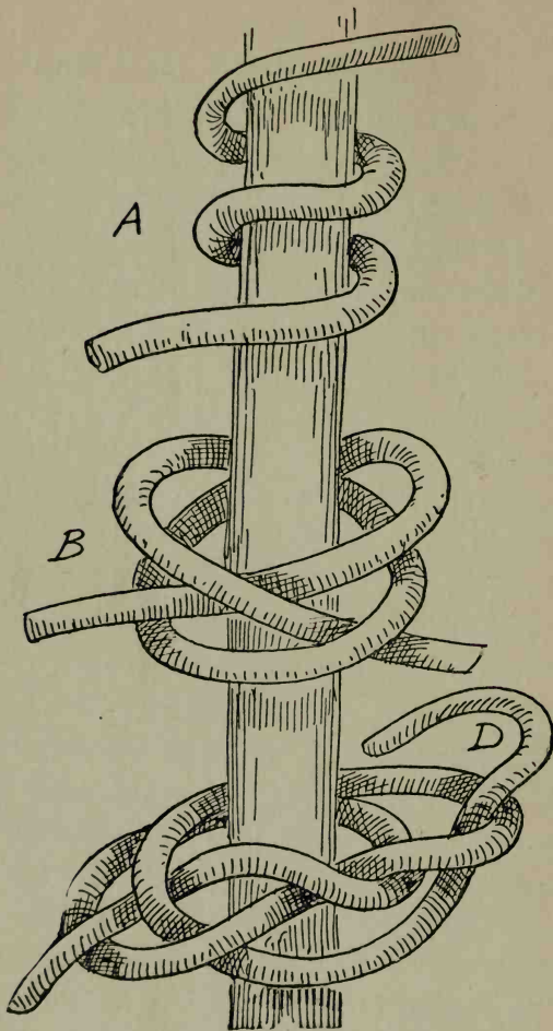
FIG. 135.—Making Turk's head.
